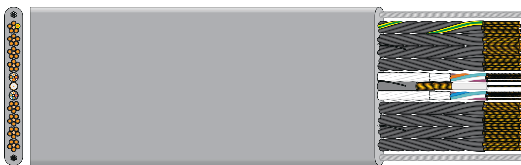
Drawing according to article number 161448 - Type 8292-F
